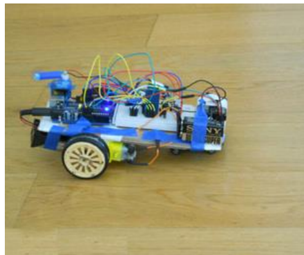
REMOTE CONTROLLED ARDUINO CAR
